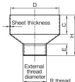
A10685 Stainless steel A-type hopper, external thread (SUS 304)
