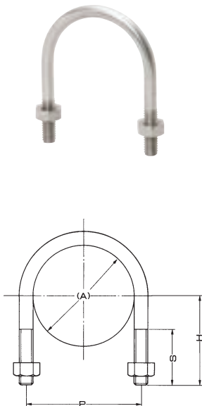
Part number A10617 Stainless steel U-bolt
