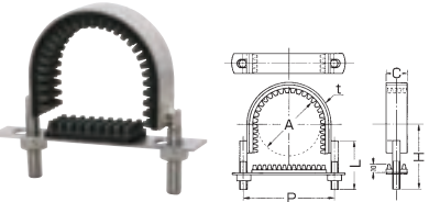
Anti-vibration stainless steel U-band with plate
