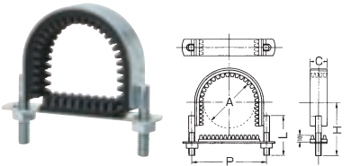
Anti-vibration U-band with plate
