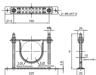
Basic dimension drawing
