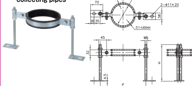
Upper support for collecting pipes
