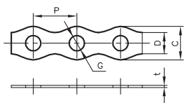
Part number A10246 Stainless steel Type B suspension band
