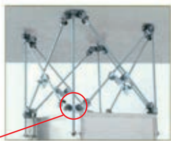
Example of anti-sway L-fitting installation
